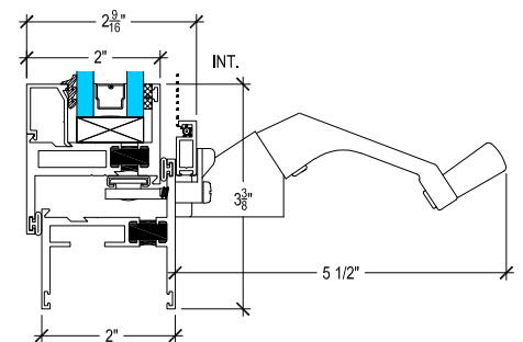
SILL
