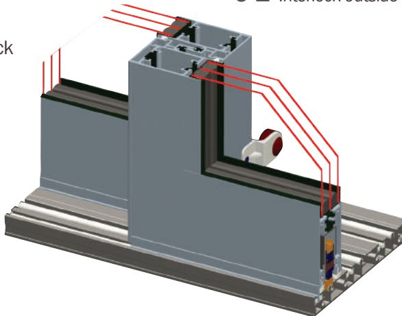
C-1 Interlock outside view
