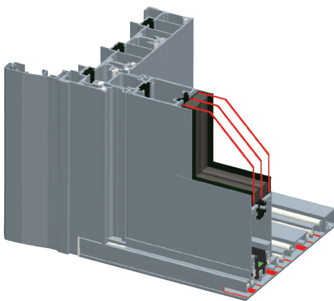
B Fixed panel lower corner, outside view
