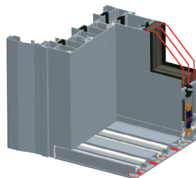
B MTS door moving panel outside view
