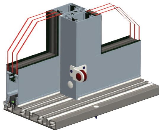
C-2 Interlock inside view
