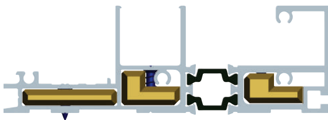
Mainframe and connector sectional view
