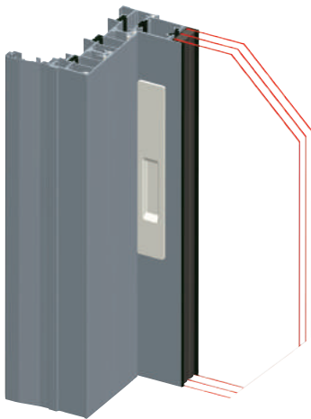
A MTS door handle and locking system, outside view
