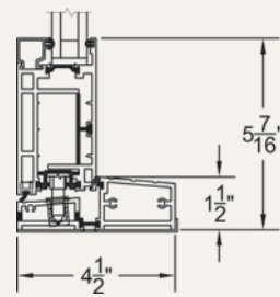
Sill
