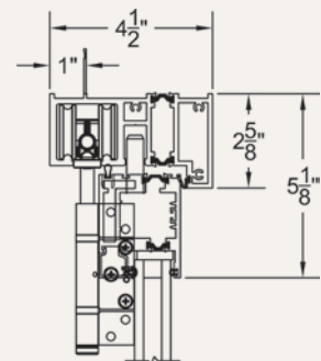
Head
